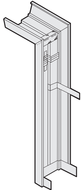
CORNER ASSEMBLY & ANCHORS
